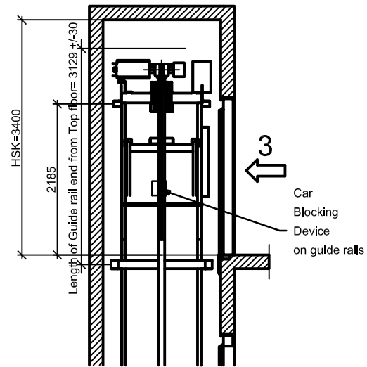
CW vertical Section: 1:50
